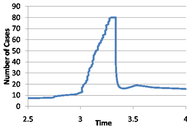
Fig. 7. Distribution of Test Cases against Pathfinding Time (in seconds) – Case B.
