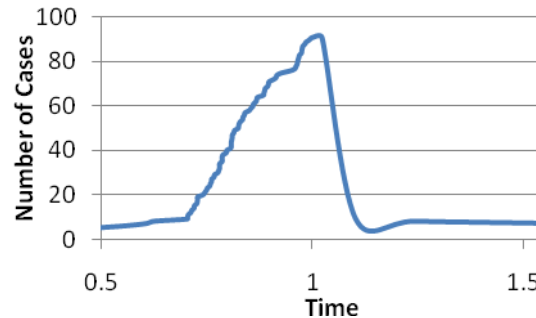
Fig. 6. Distribution of Test Cases against Pathfinding Time (in seconds) – Case A.
